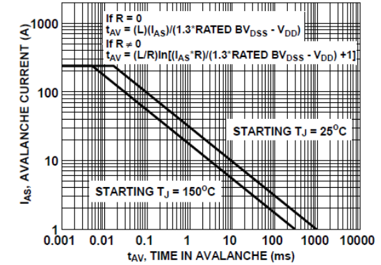
Figure 4. Unclamped Inductive Switching Capability
